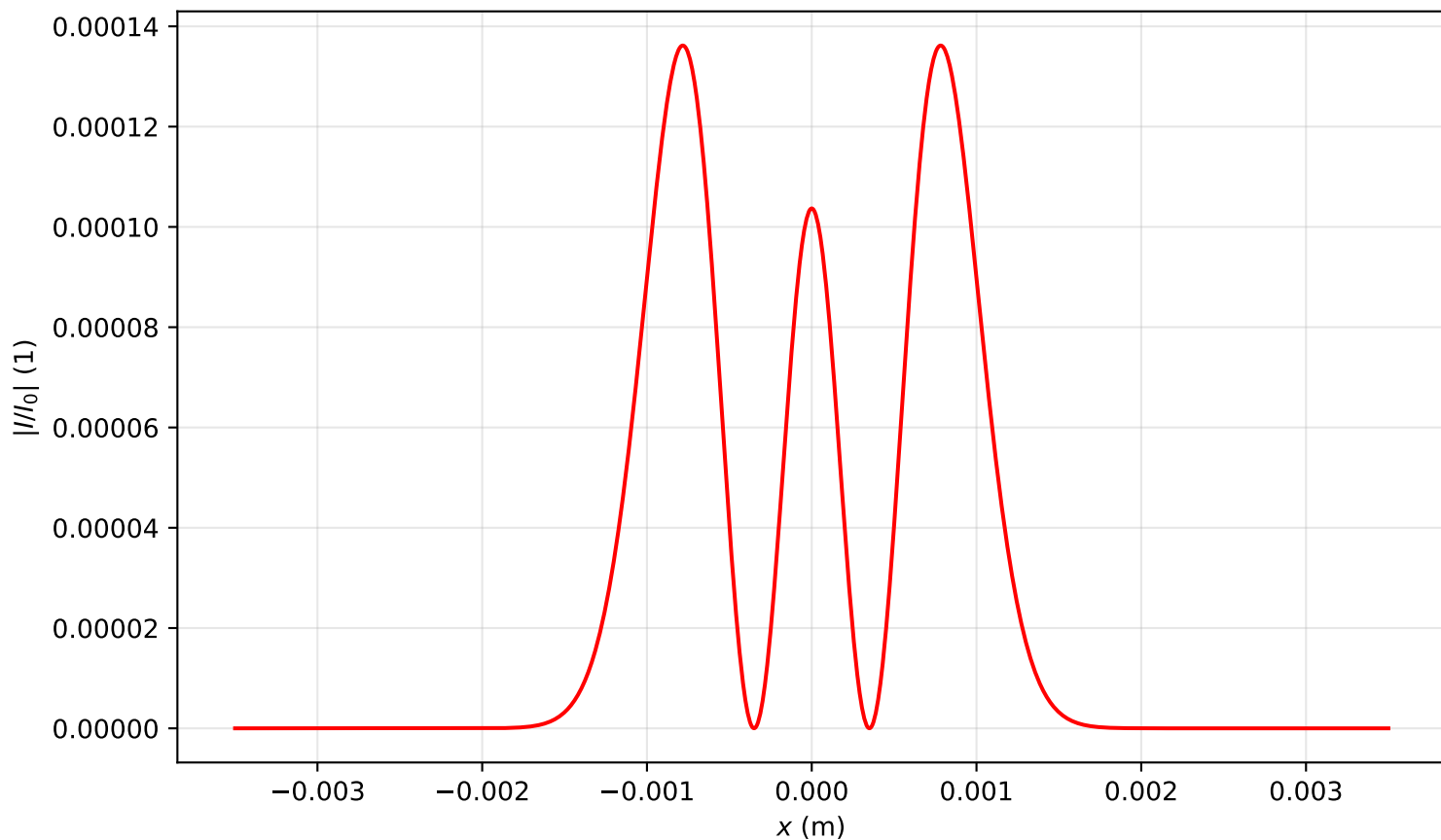
Intensity profile I(x, y = 0, z = 0.000)/I_0 , P_{in}=1.0P_{cr} , artificial time
